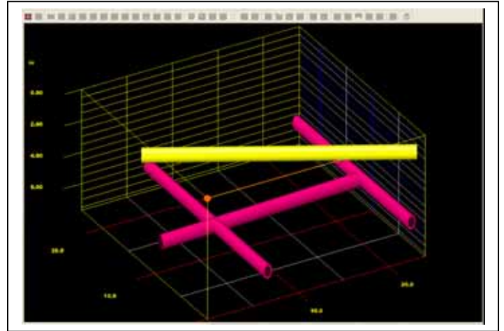
Images show electrical conduit above rebar.
